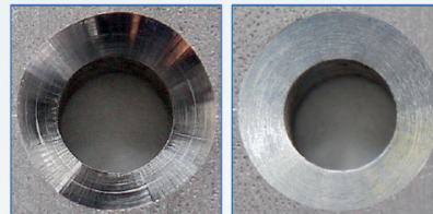
Standard-Senker 42CrMo, v_c = 15 \text{ m/min} , f_u = 0.15
