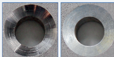
Standard-Senker 42CrMo, v_c = 15 \text{ m/min} , f_u = 0.15
