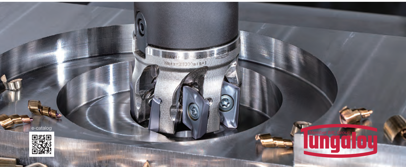
AV*T18 Max. depth of cut: 16.5 mm AV*T12 Max. depth of cut: 11.5 mm
